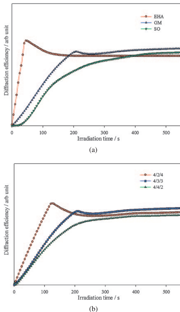
Figure 1. Real time diffraction efficiency as a function of irradiation time for various types of monofunctional reactive diluents (a) and at various compositions of GM (b) in a developing HPDLC grating (irradiated at 633 nm).
